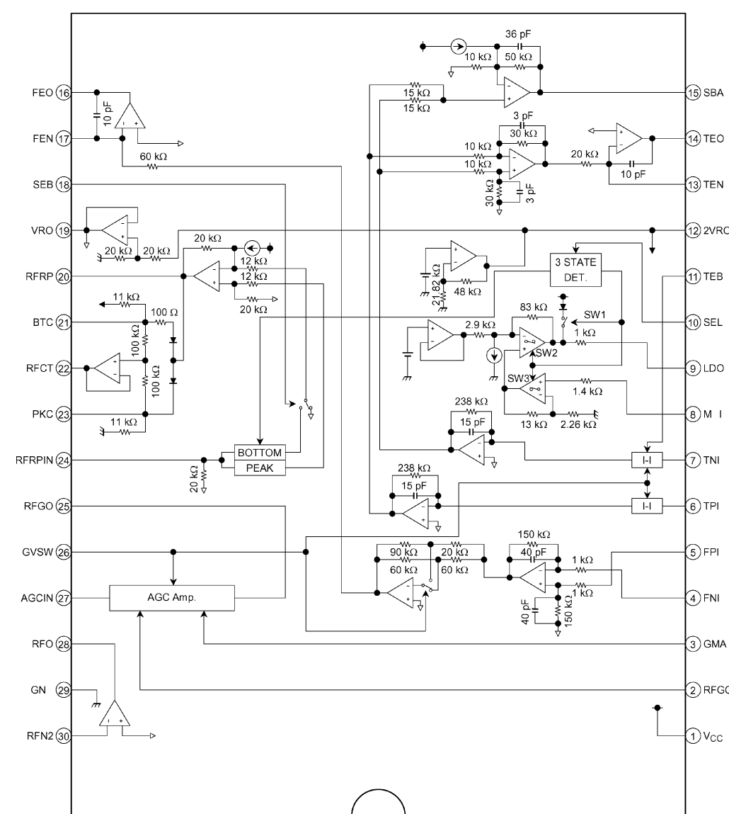
IC702 / TA2153FN
